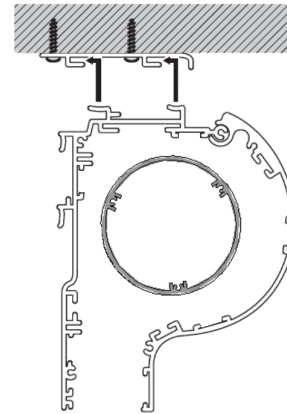
Ceiling Mounting
